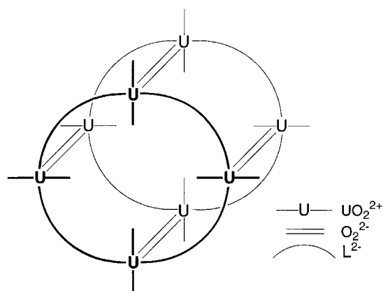
Scheme 1 Schematic representation of the anionic complex core in 1 .
