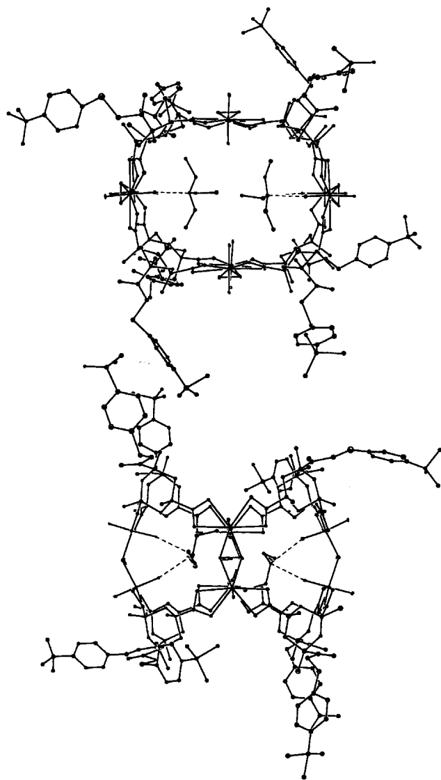
Fig. 2 Two orthogonal views of the structure of 1 . All counter ions and solvent molecules omitted other than the two triethylammonium ions included in the cavity. Hydrogen bonds between nitrogen and uranyl oxygen atoms in dashed lines. Top view parallel to the larger face defined by a (\text{UO}_2\text{L})_4 macrocoring. Lower view showing the coordination geometry around uranyl ions and the bridging \mu -peroxo ions.
