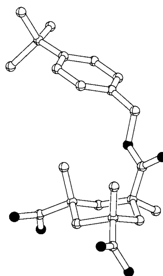
Fig. 1 View of the ligand L 2- in the uranyl complex 1 . Oxygen atoms in black.
